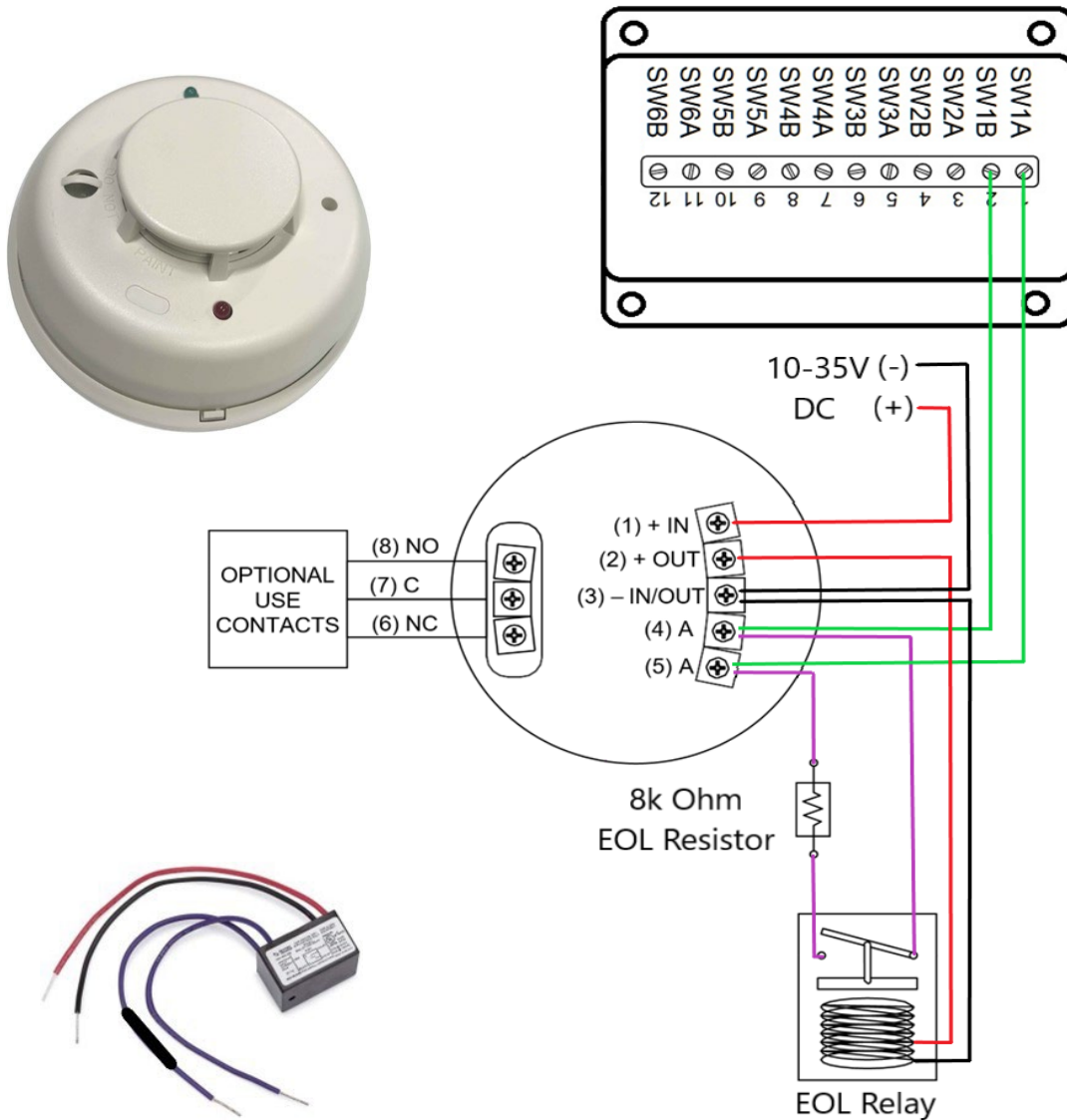
Figure 1 - Wiring Diagram
