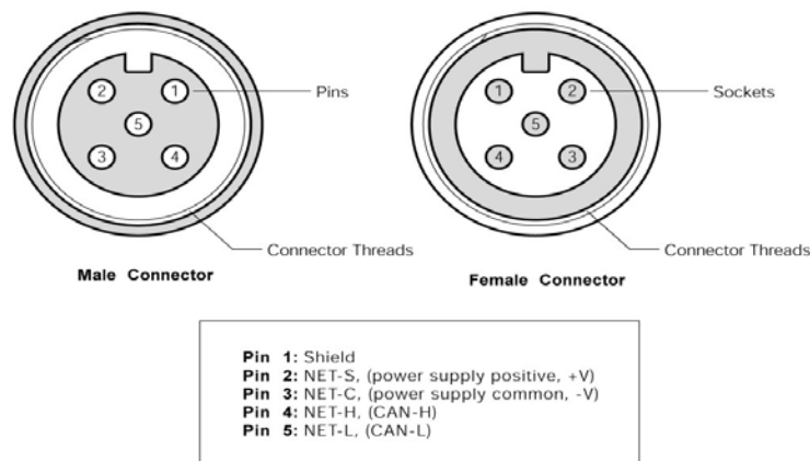
Figure 2 – NMEA 2000® Connector Face Views
