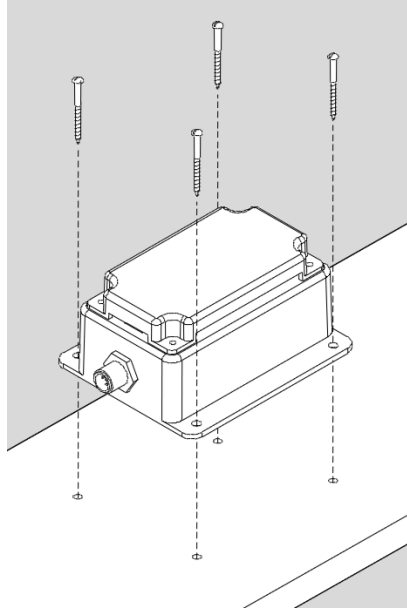
Figure 1 – Mounting the SIM100
