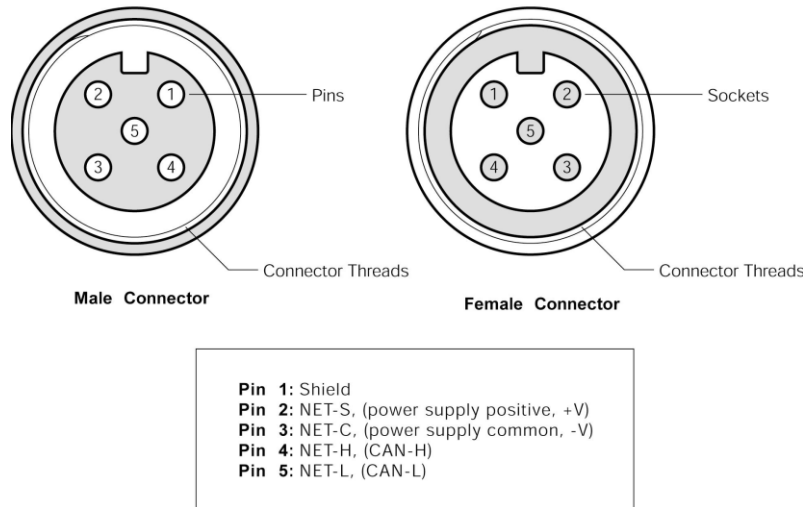
Figure 7 – NMEA 2000® Connector Face Views
