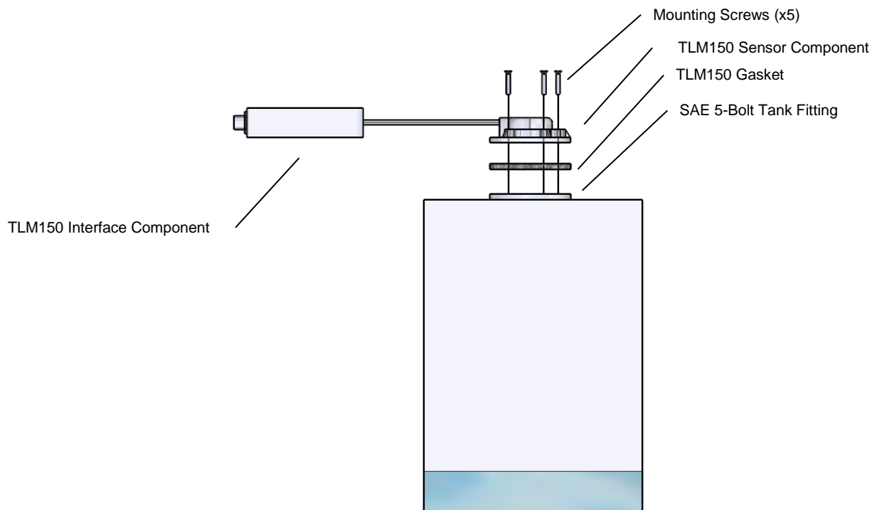
Figure 2 – TLM150 Mounting – SAE 5-Hole Bolt Pattern
