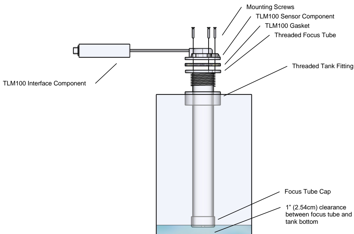
Figure 5 – Mounting TLM100 with Focus Tube on Threaded Tank Fitting
