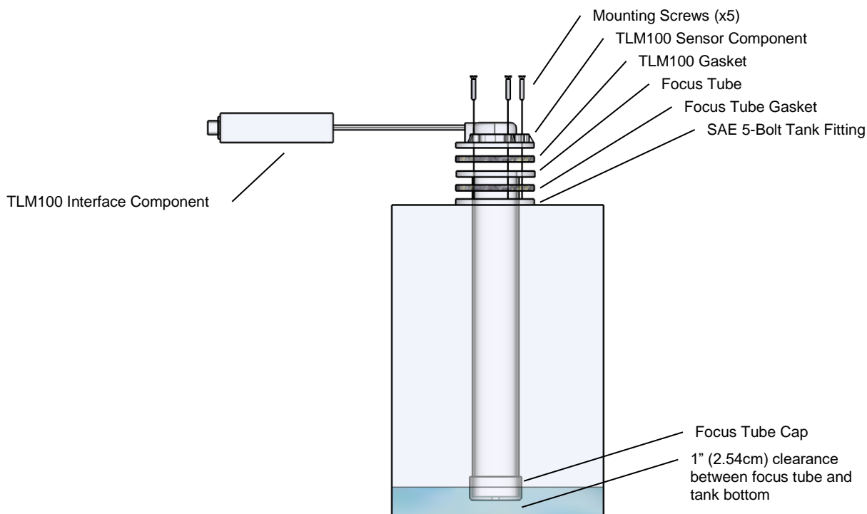
Figure 3 – Mounting TLM100 to SAE 5-Hole Tank with Focus Tube
