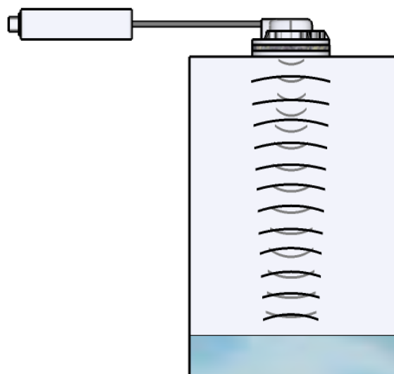
Figure 1 – TLM100 Operation
