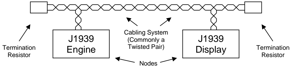
Figure 2 - Typical Single Engine J1939 Network
