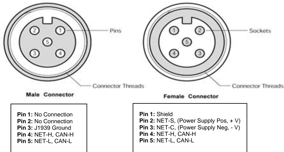
Figure 4 – J1939 Connector Face Views
