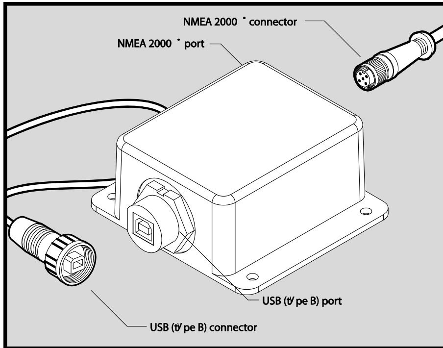
Figure 1 – Mounting the USB100
